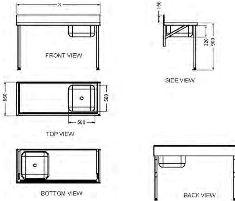
Single Bowl Catering Sink
