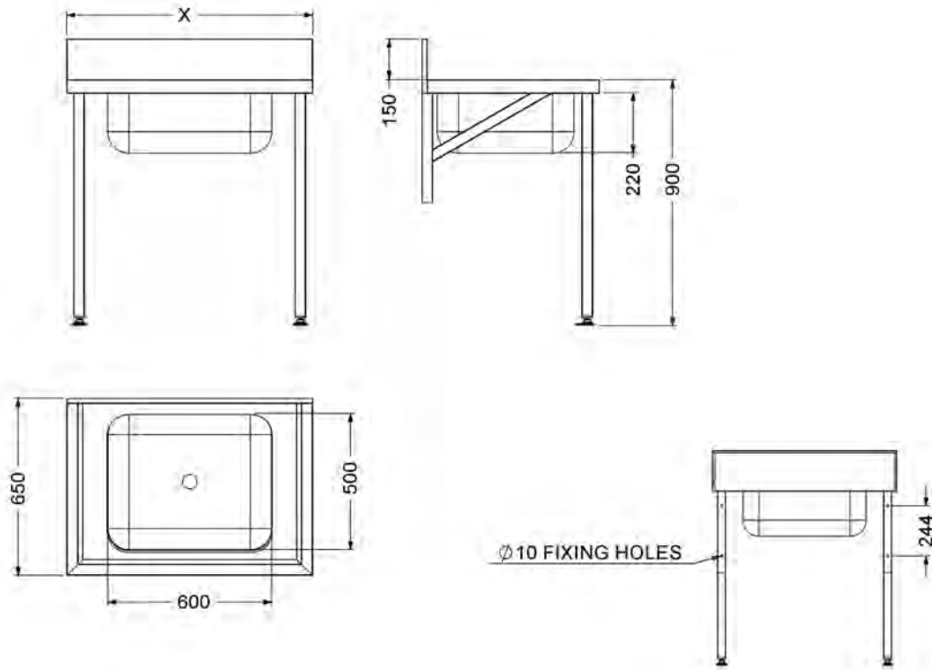
Single Bowl Pot Sink
