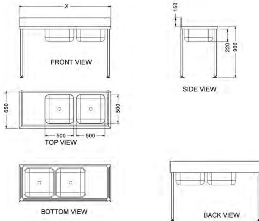
Double Bowl Catering Sink
