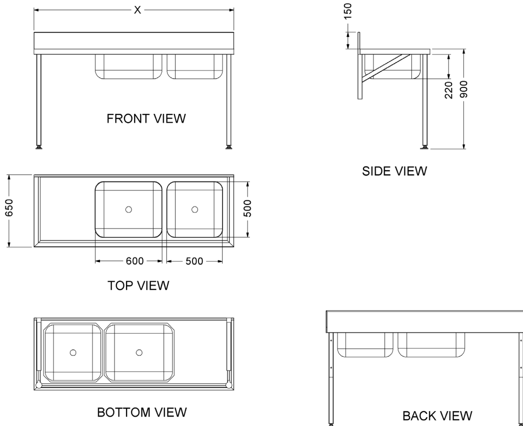
Double Bowl Pot Sink
